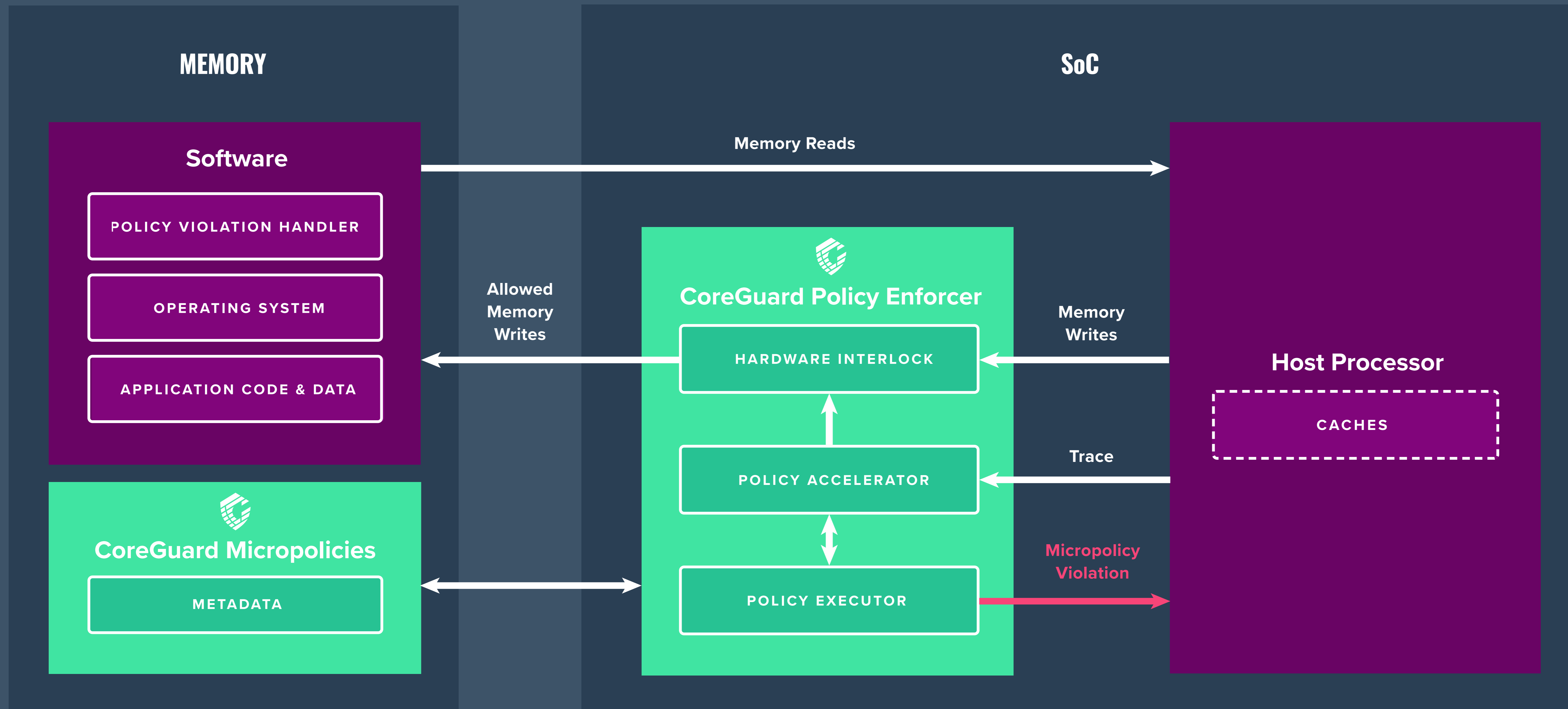
CoreGuard Block Diagram
